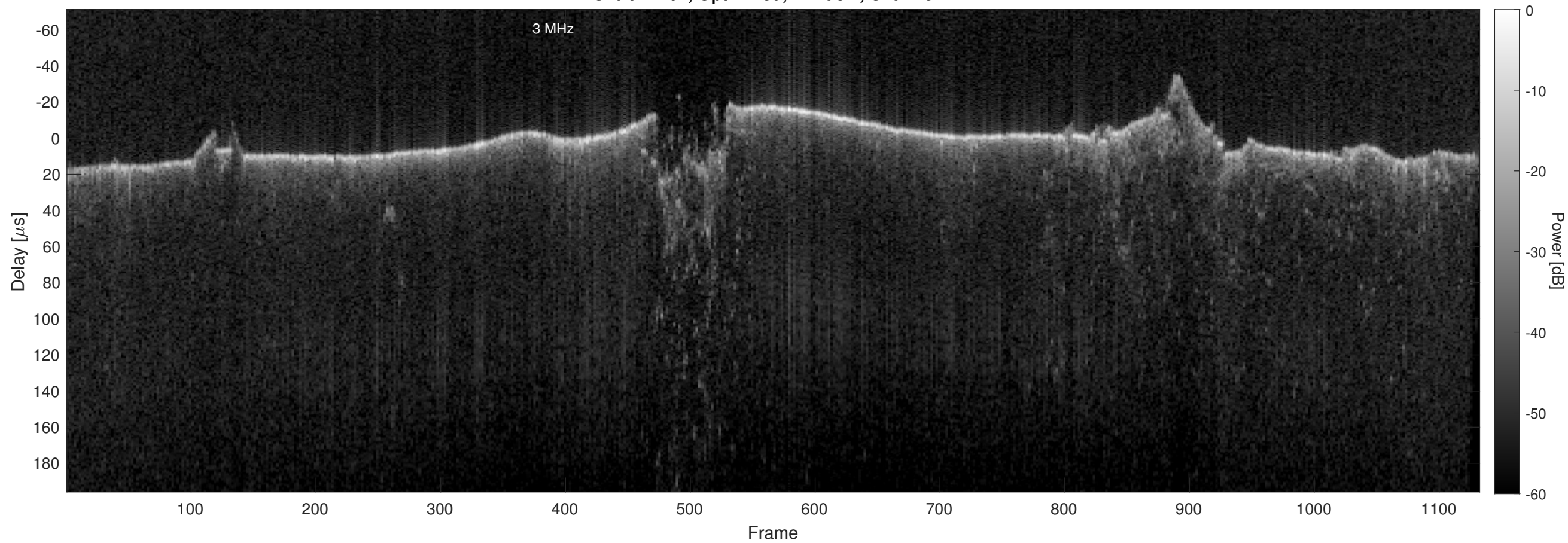
Orbit 21764, Optimized, Window, Channel 2
