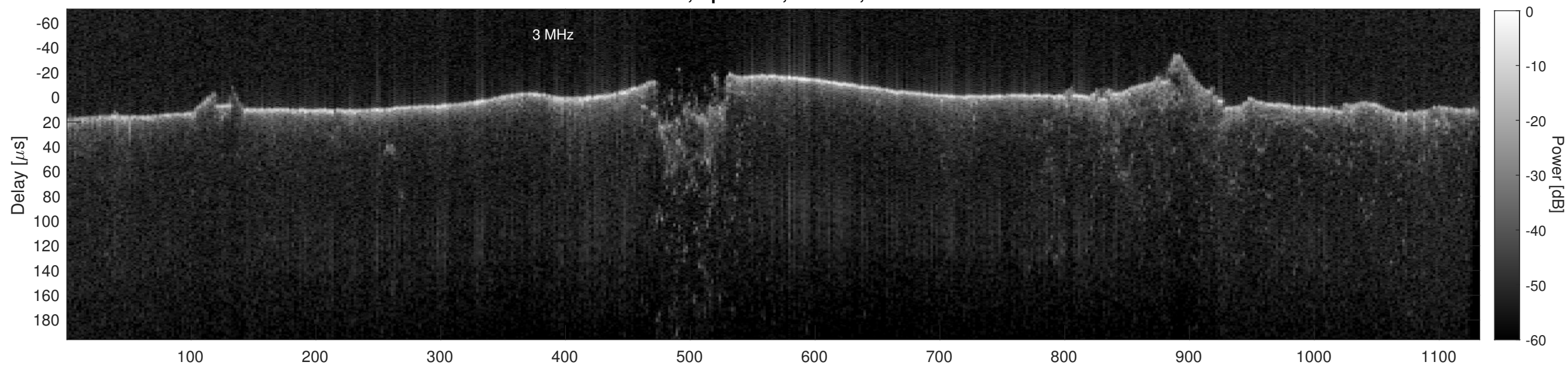
Orbit 21764, Cluttergram
