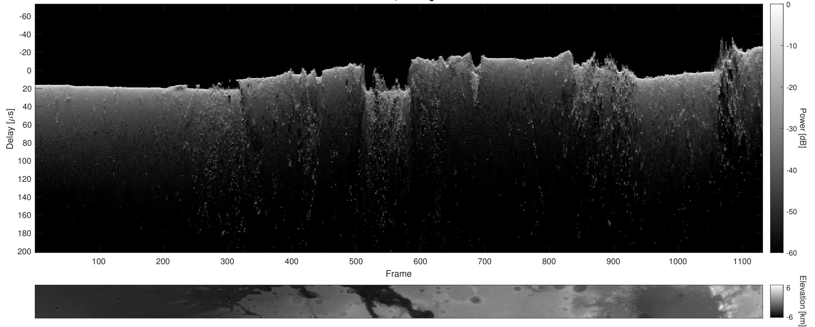
Orbit 21767, Cluttergram
