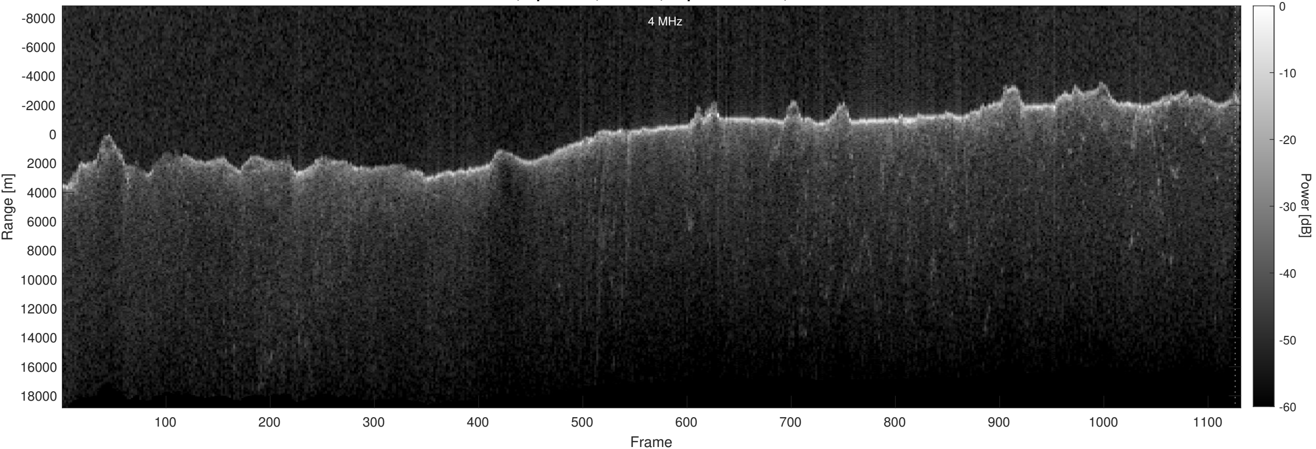
Orbit 21768, Optimized, Window, Depth-Corrected, Channel 2
