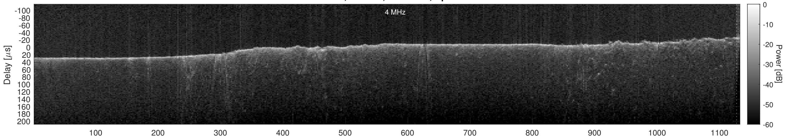
Orbit 21769, Cluttergram
