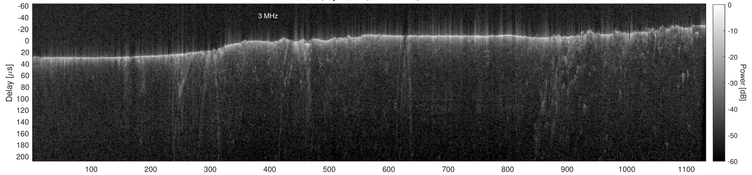
Orbit 21769, Cluttergram
