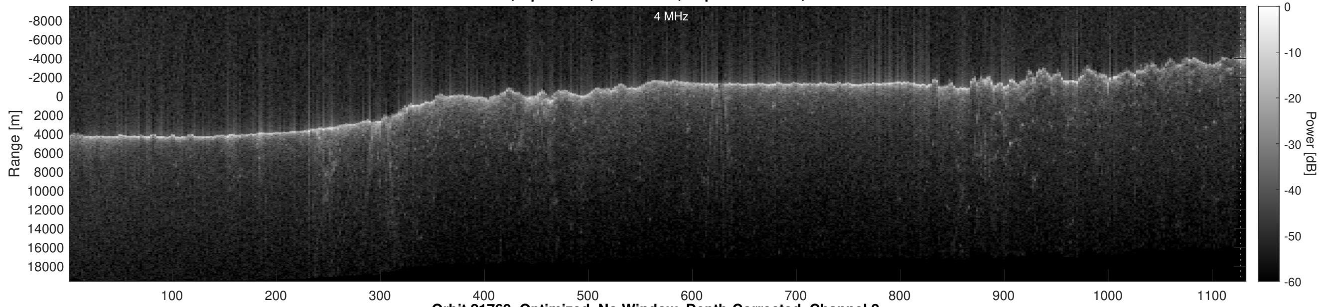
Orbit 21769, Optimized, No Window, Depth-Corrected, Channel 2
