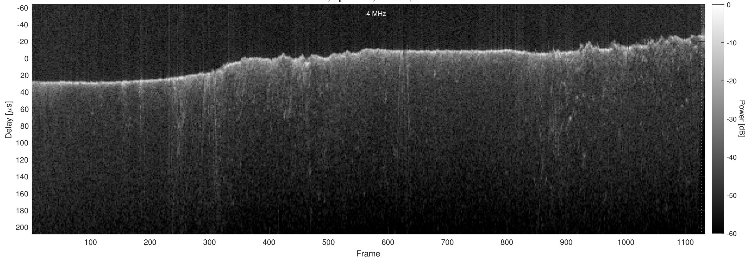
Orbit 21769, Optimized, Window, Channel 2
