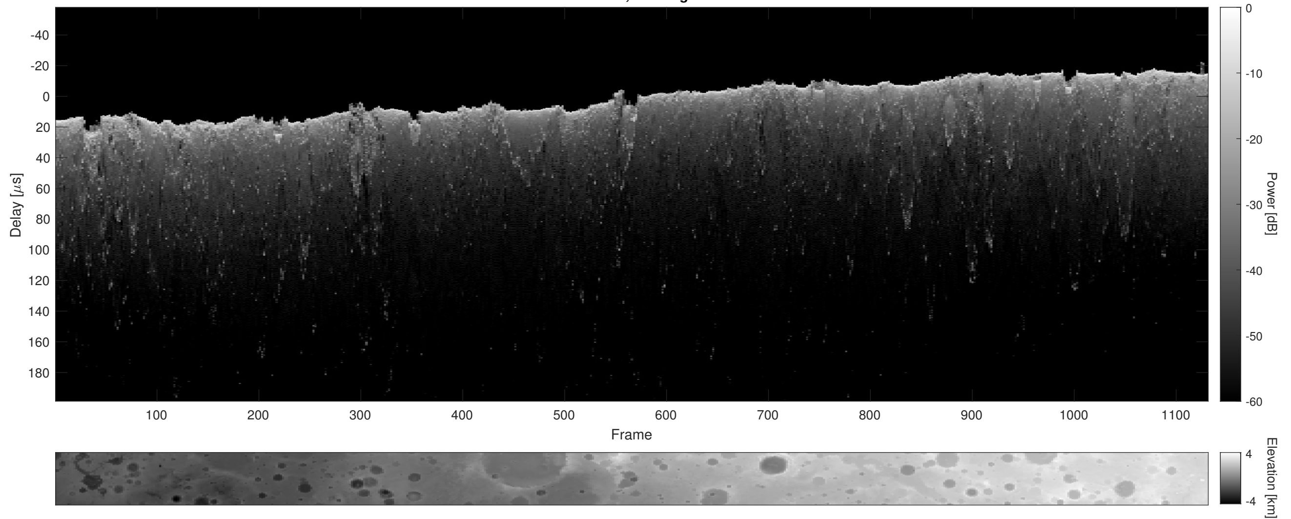
Orbit 21770, Cluttergram
