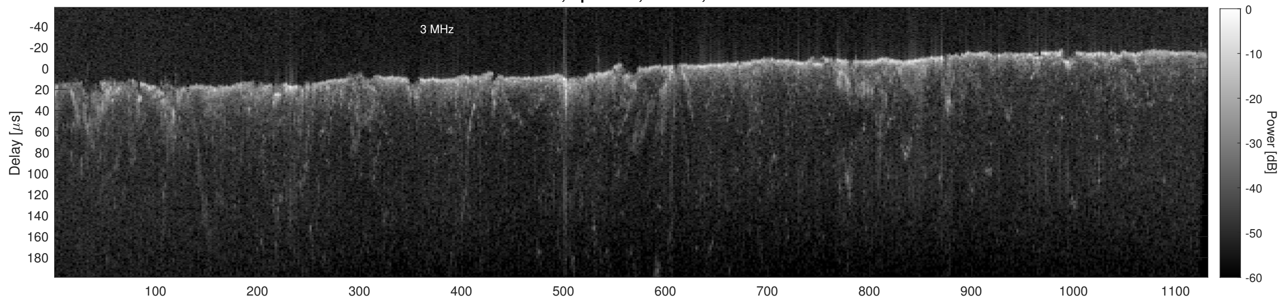
Orbit 21770, Cluttergram
