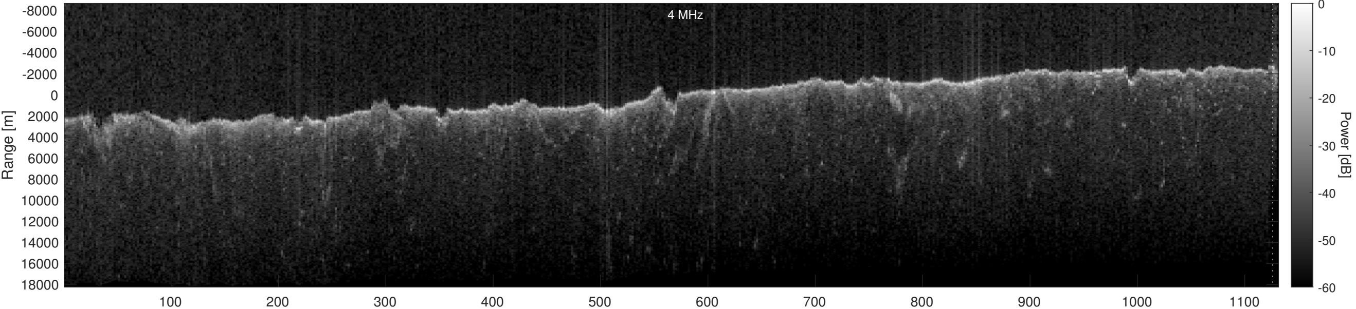
Orbit 21770, Optimized, Window, Depth-Corrected, Channel 2
