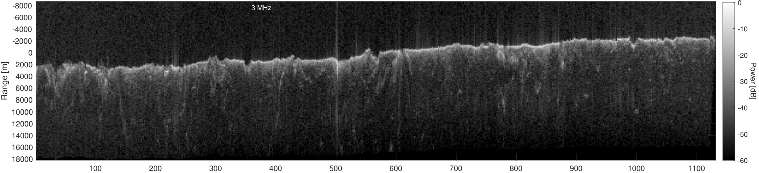
Orbit 21770, Depth-Corrected Cluttergram
