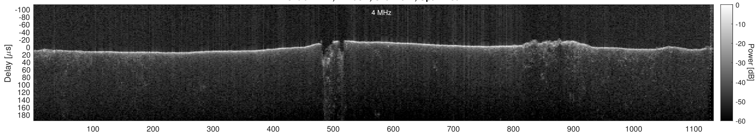
Orbit 21771, Cluttergram
