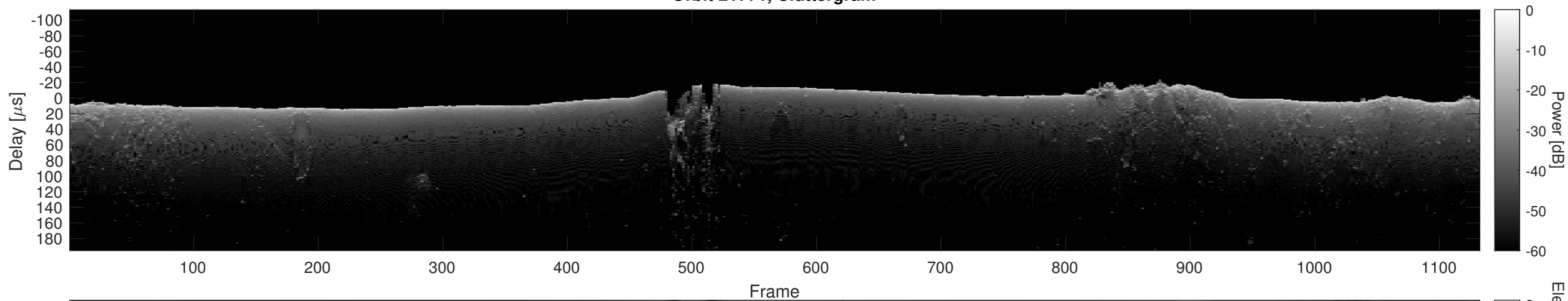
Orbit 21771, Cluttergram
