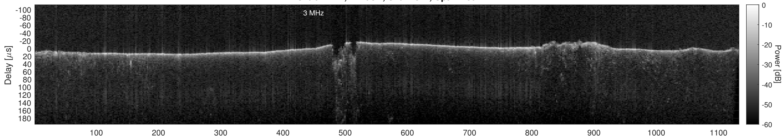
Orbit 21771, Cluttergram
