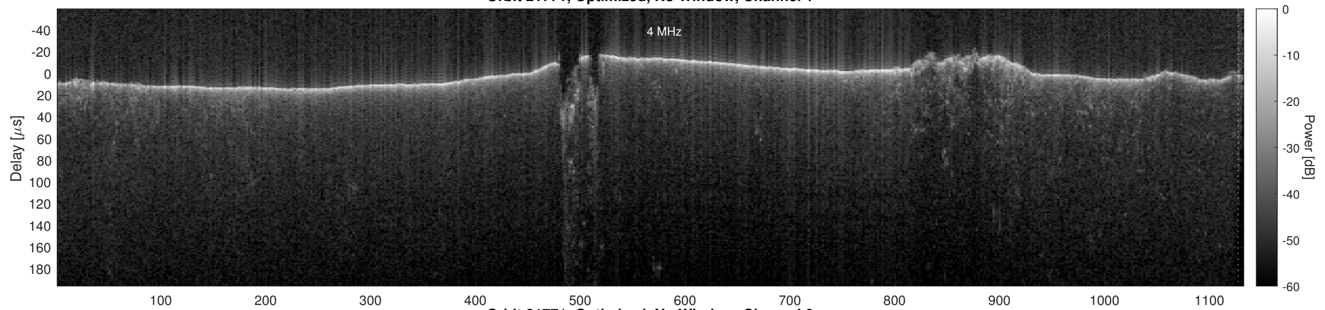
Orbit 21771, Optimized, No Window, Channel 2
