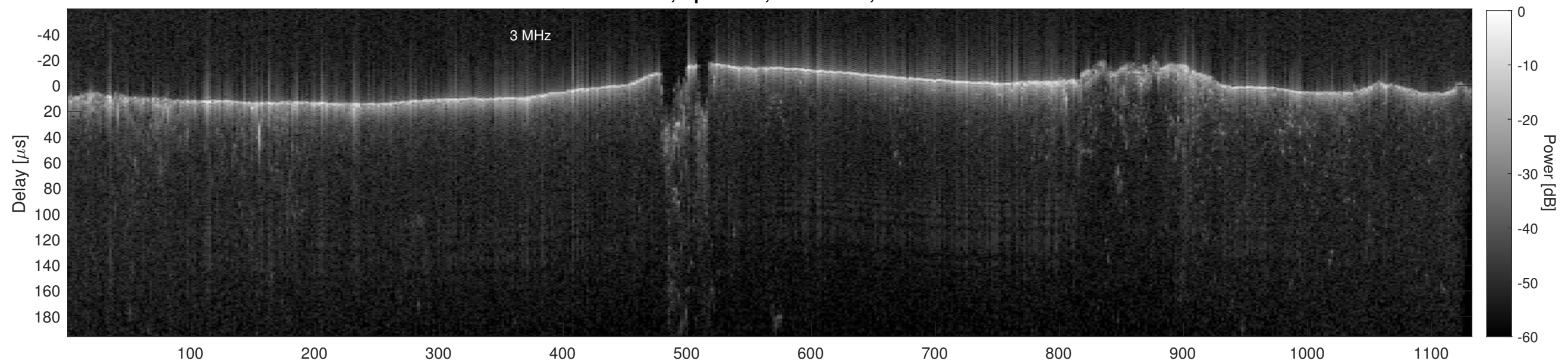
Orbit 21771, Cluttergram
