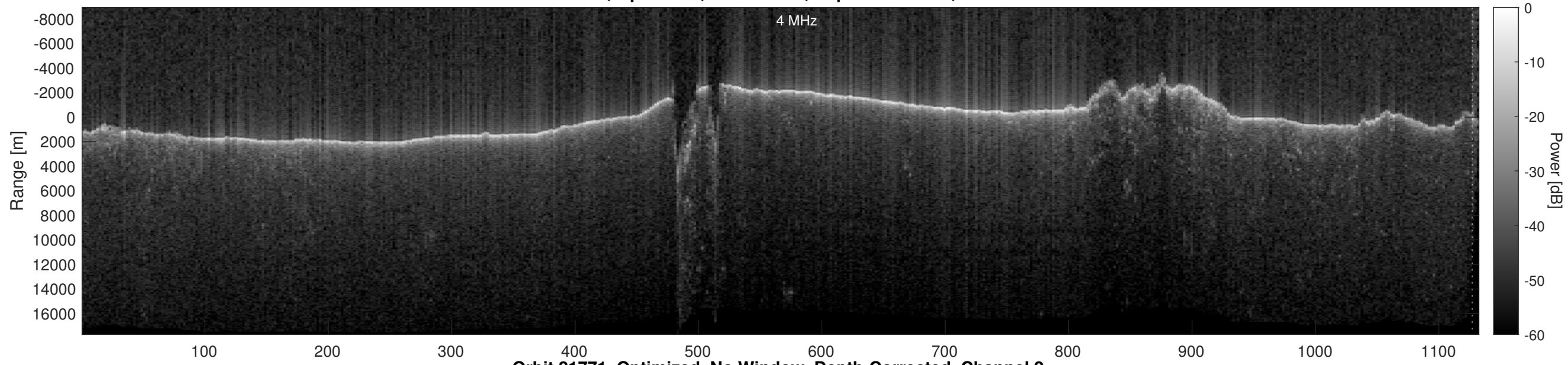
Orbit 21771, Optimized, No Window, Depth-Corrected, Channel 2
