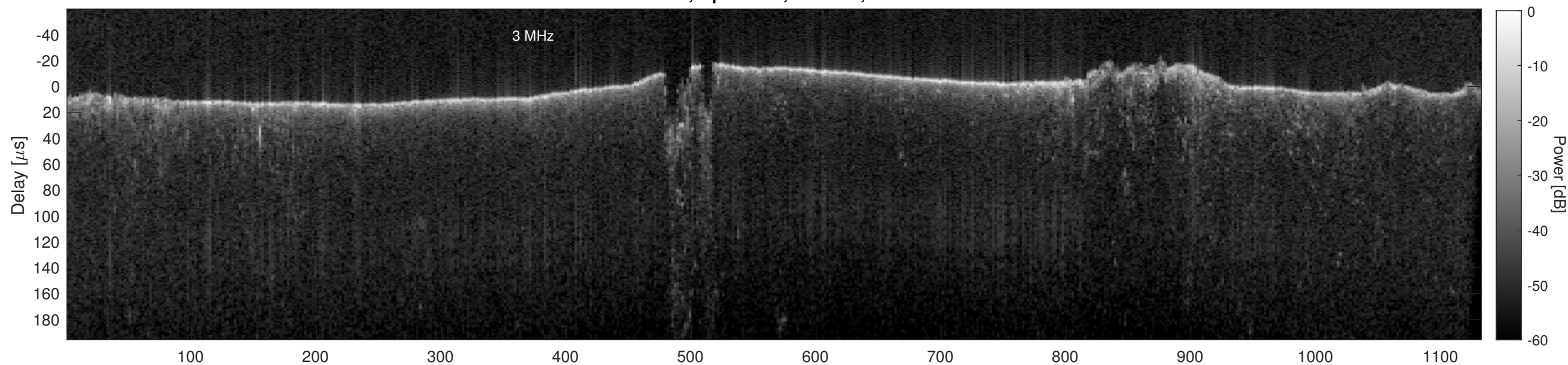
Orbit 21771, Cluttergram
