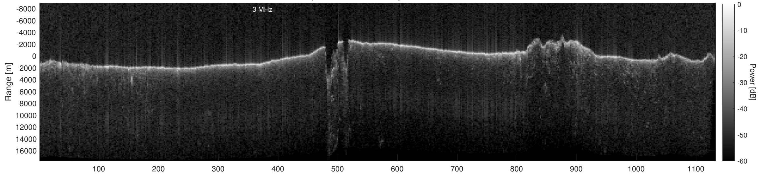
Orbit 21771, Depth-Corrected Cluttergram
