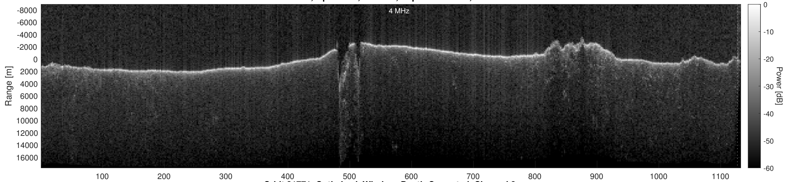
Orbit 21771, Optimized, Window, Depth-Corrected, Channel 2
