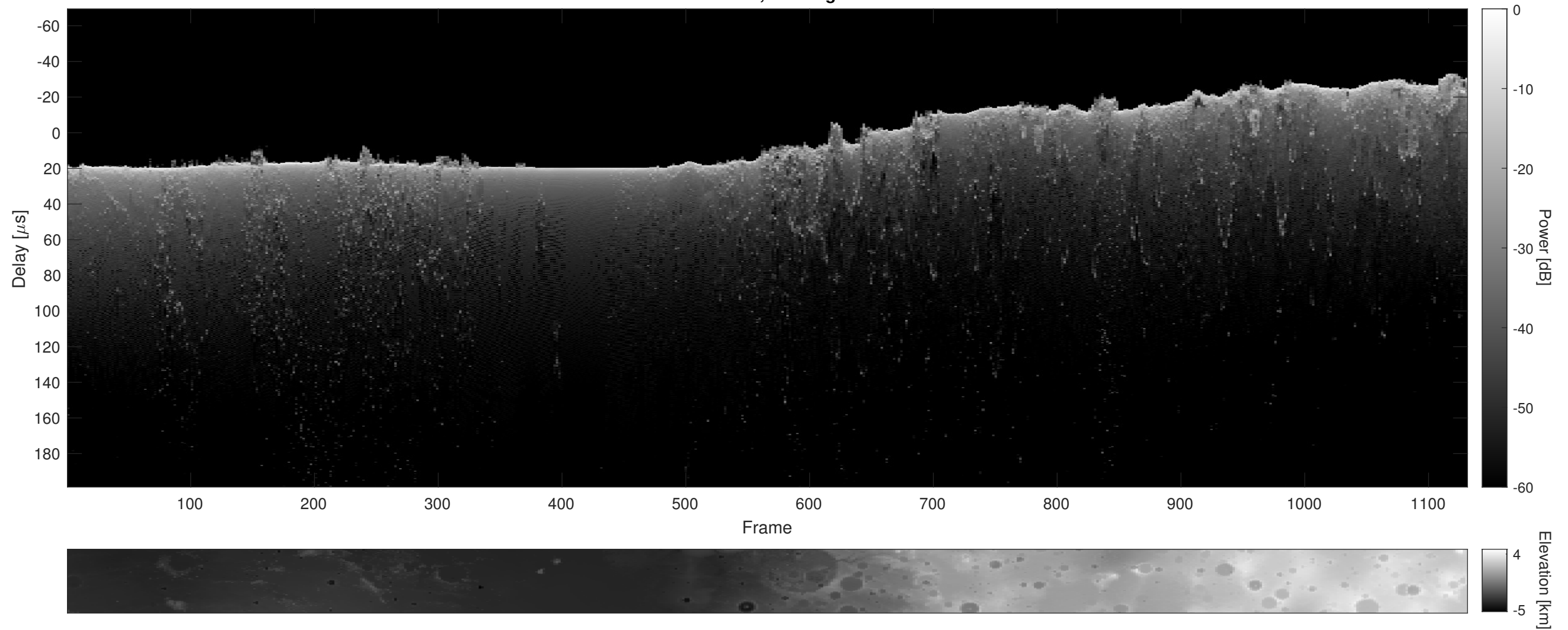
Orbit 21772, Cluttergram
