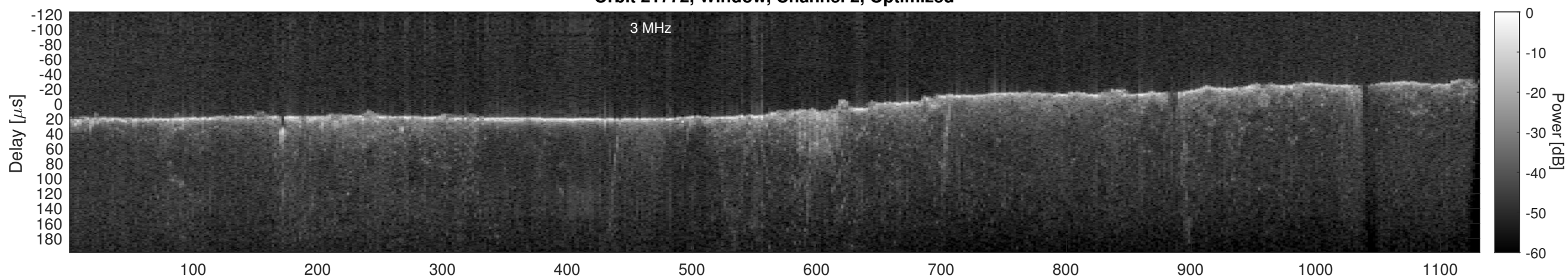
Orbit 21772, Cluttergram
