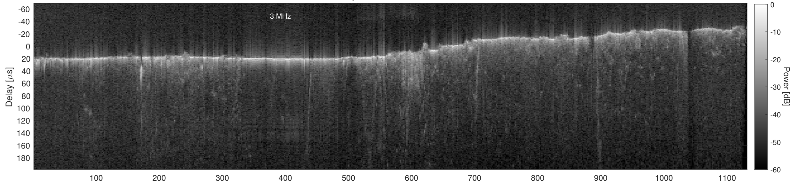
Orbit 21772, Cluttergram
