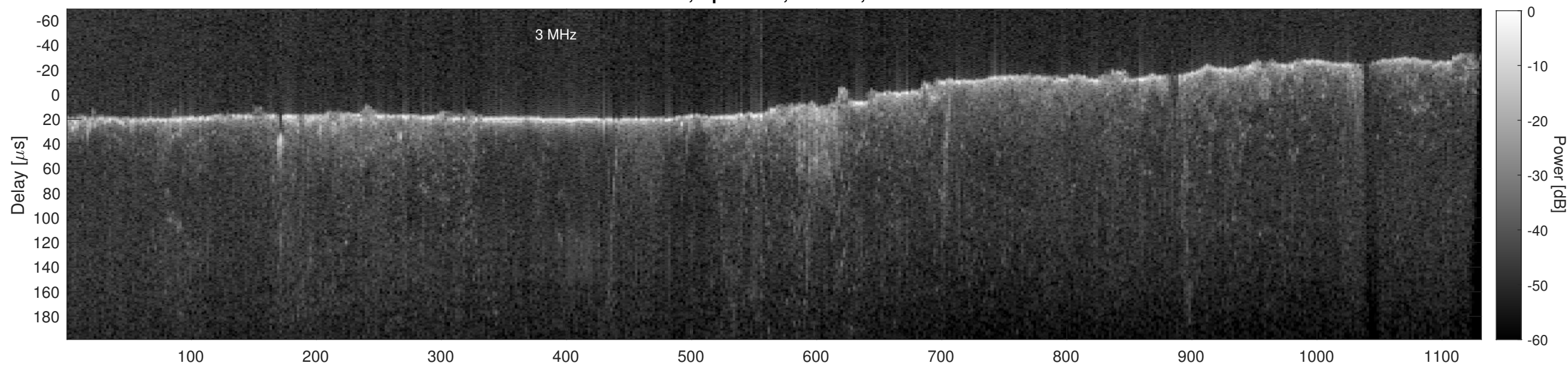
Orbit 21772, Cluttergram
