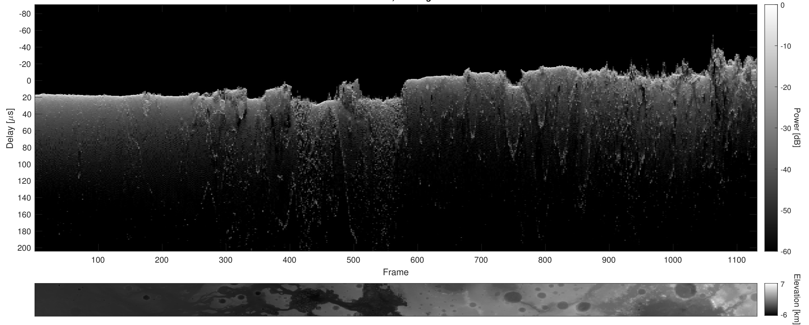
Orbit 21774, Cluttergram
