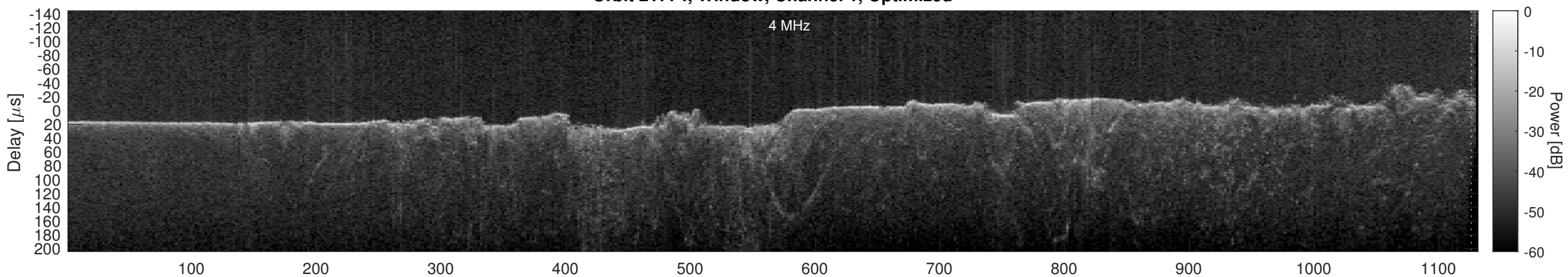
Orbit 21774, Cluttergram
