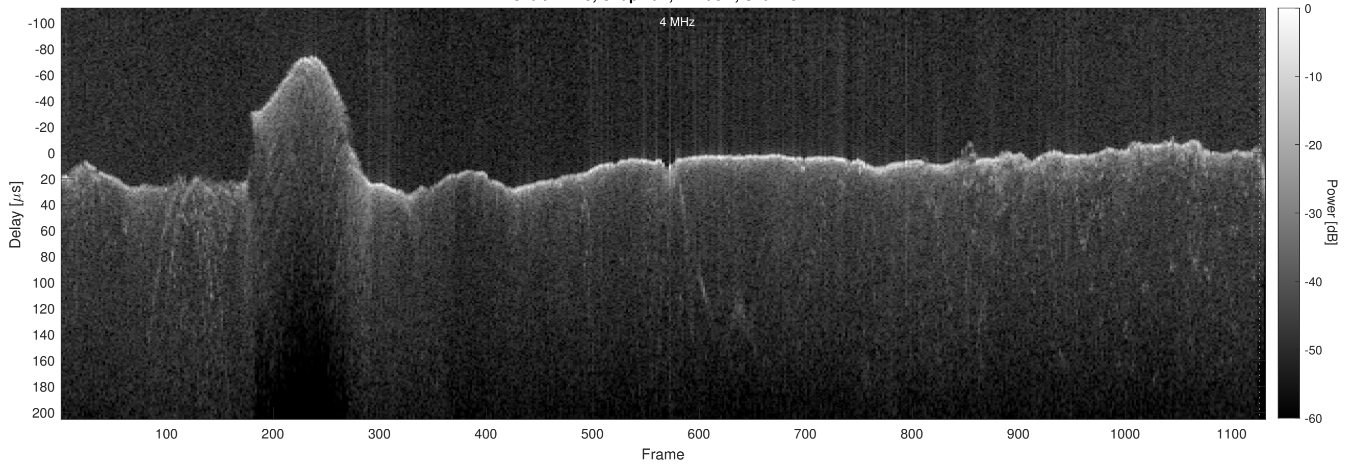
Orbit 21775, Chapman, Window, Channel 2
