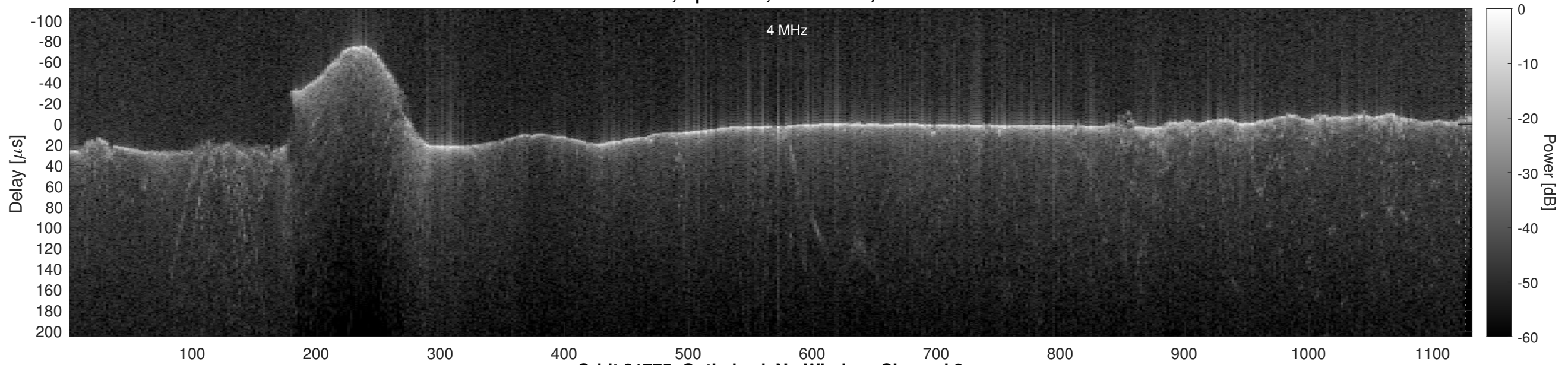
Orbit 21775, Optimized, No Window, Channel 2
