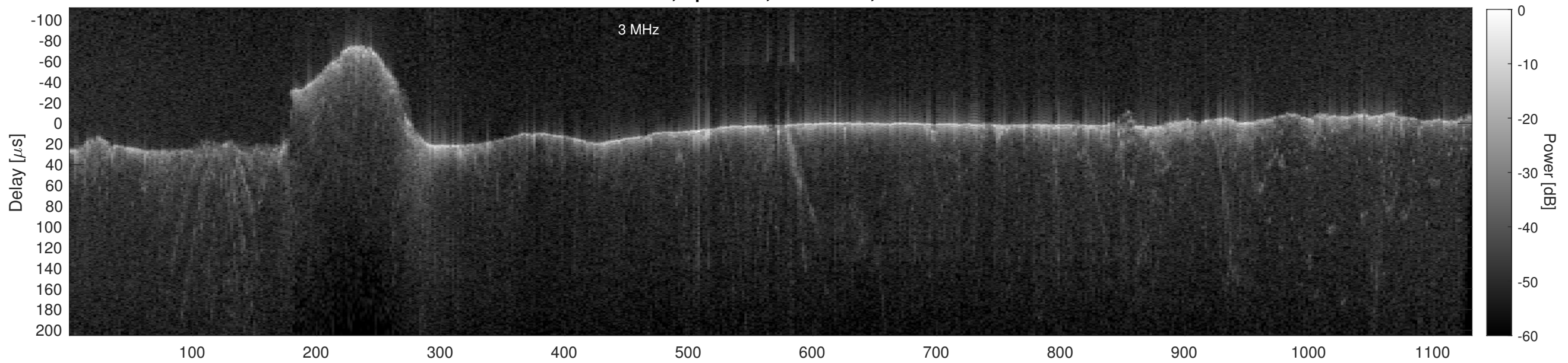
Orbit 21775, Cluttergram
