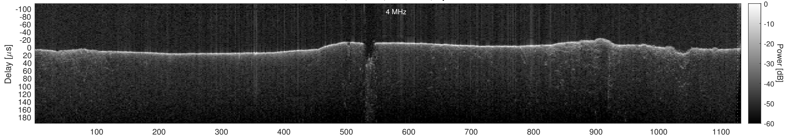
Orbit 21778, Cluttergram
