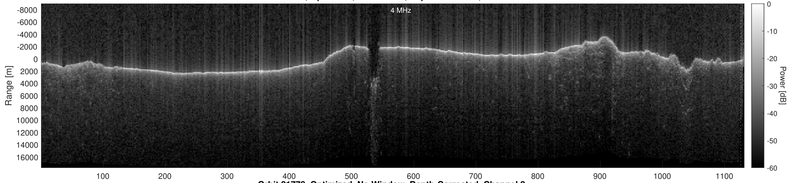
Orbit 21778, Optimized, No Window, Depth-Corrected, Channel 2
