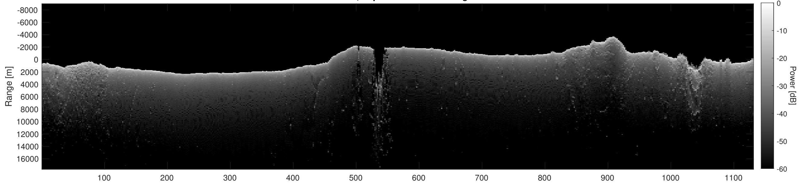
Orbit 21778, Depth-Corrected Cluttergram
