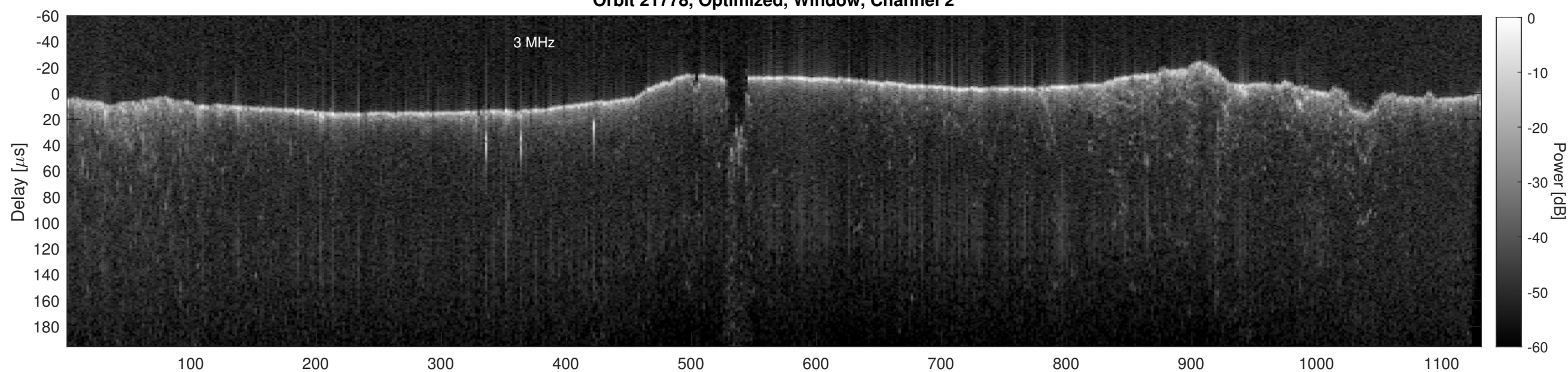
Orbit 21778, Cluttergram
