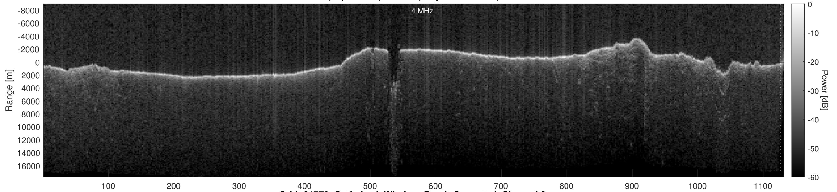
Orbit 21778, Optimized, Window, Depth-Corrected, Channel 2
