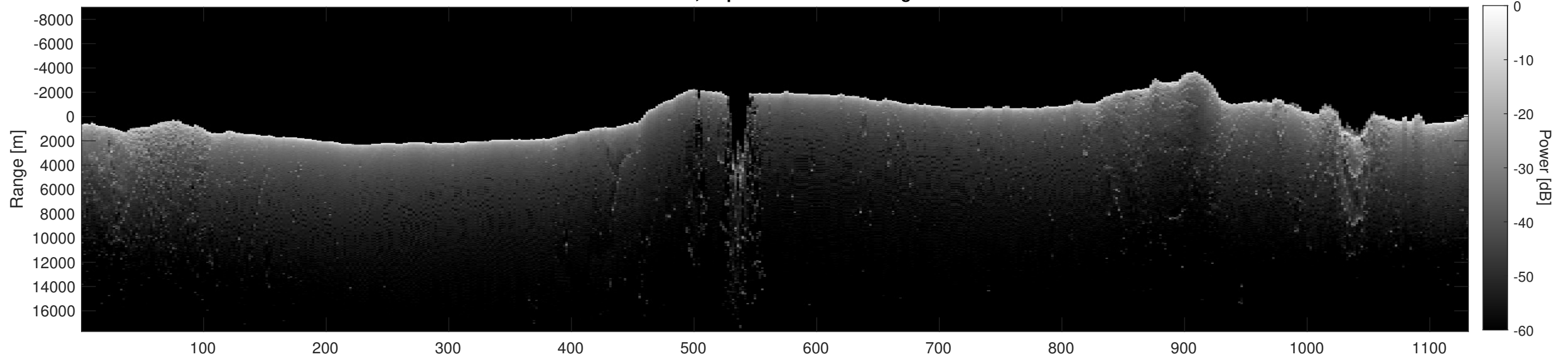
Orbit 21778, Depth-Corrected Cluttergram
