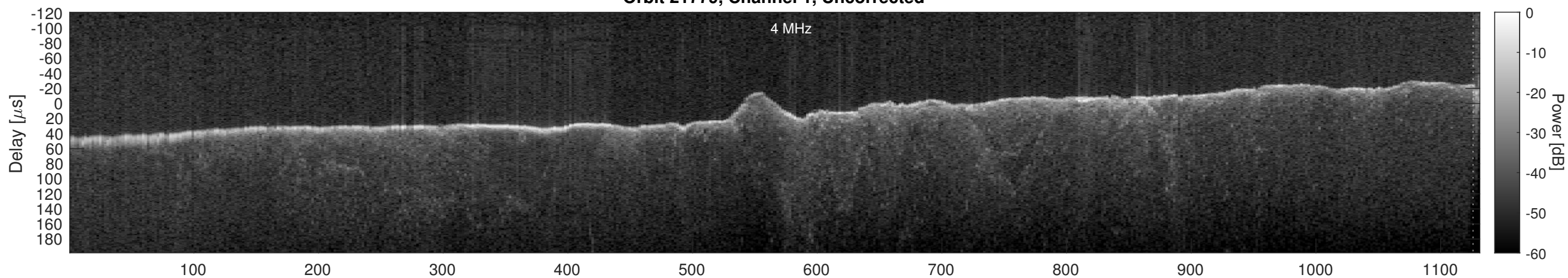
Orbit 21779, Window, Channel 1, Chapman
