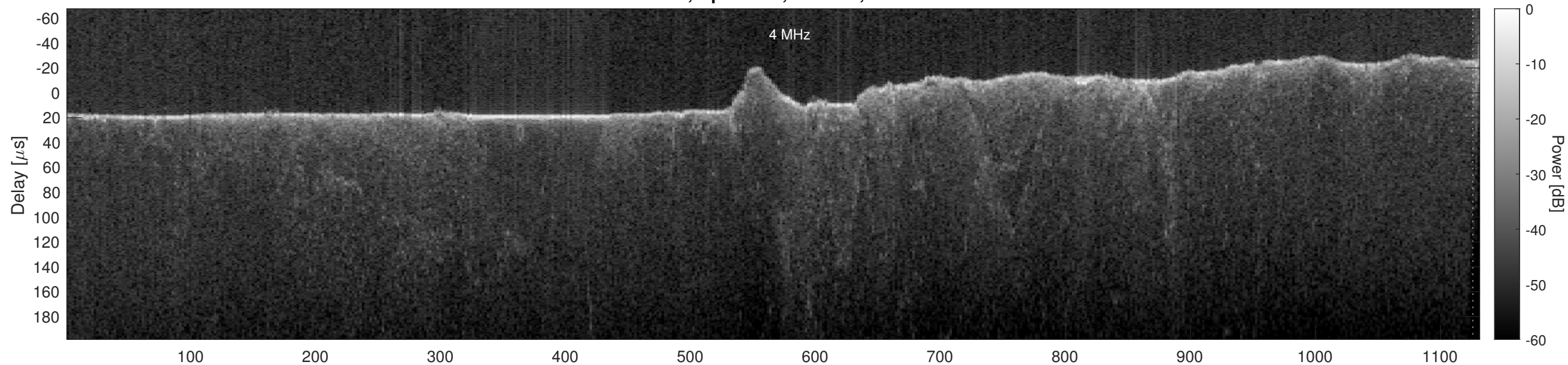
Orbit 21779, Optimized, Window, Channel 2
