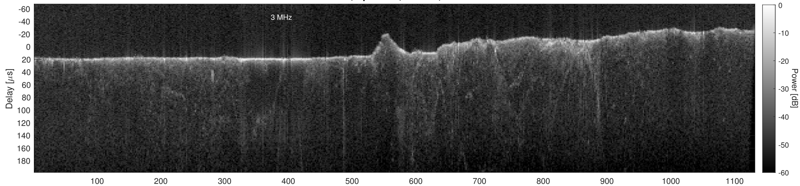
Orbit 21779, Cluttergram
