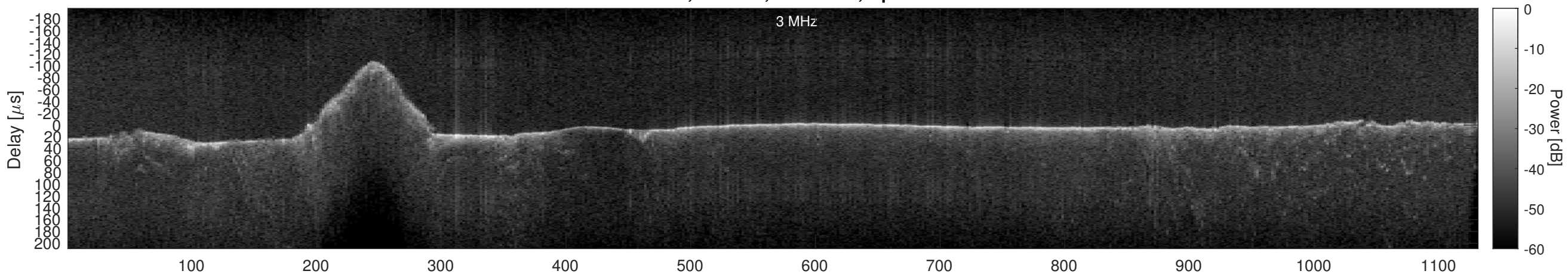
Orbit 21782, Cluttergram
