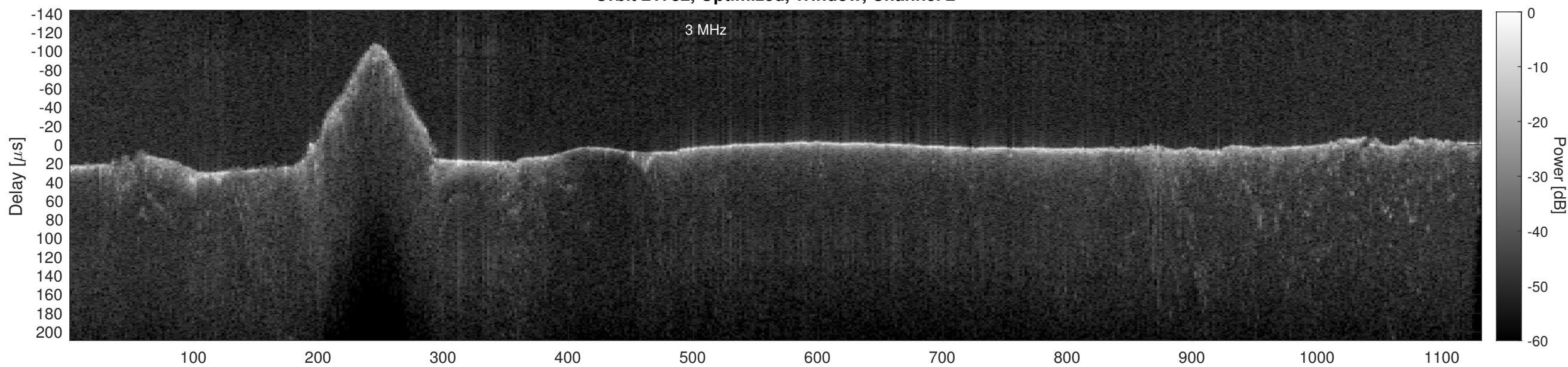
Orbit 21782, Cluttergram
