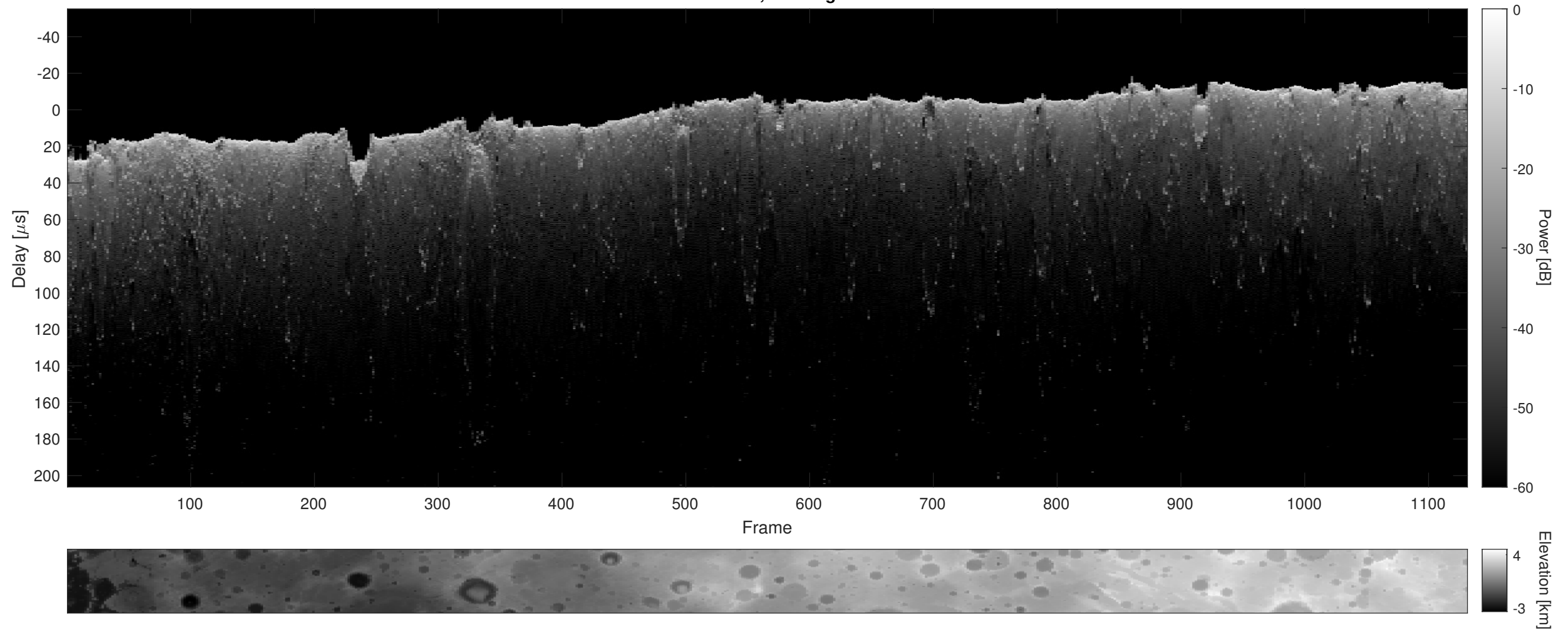
Orbit 21784, Cluttergram
