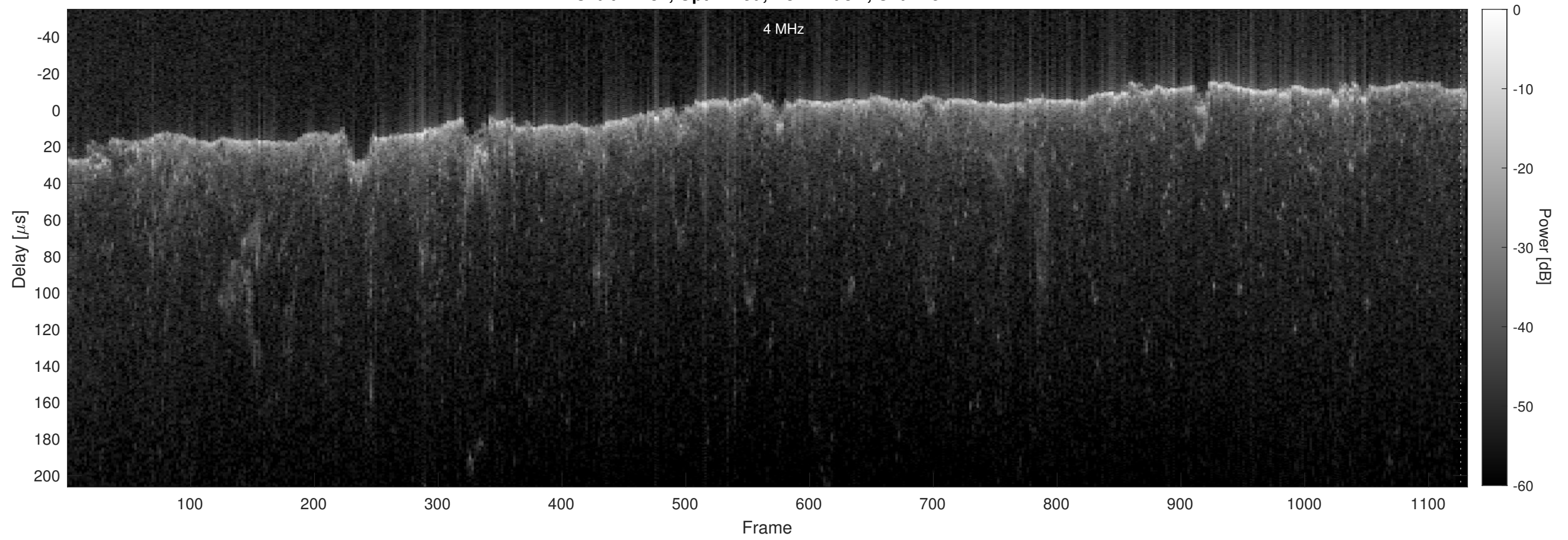
Orbit 21784, Optimized, No Window, Channel 2
