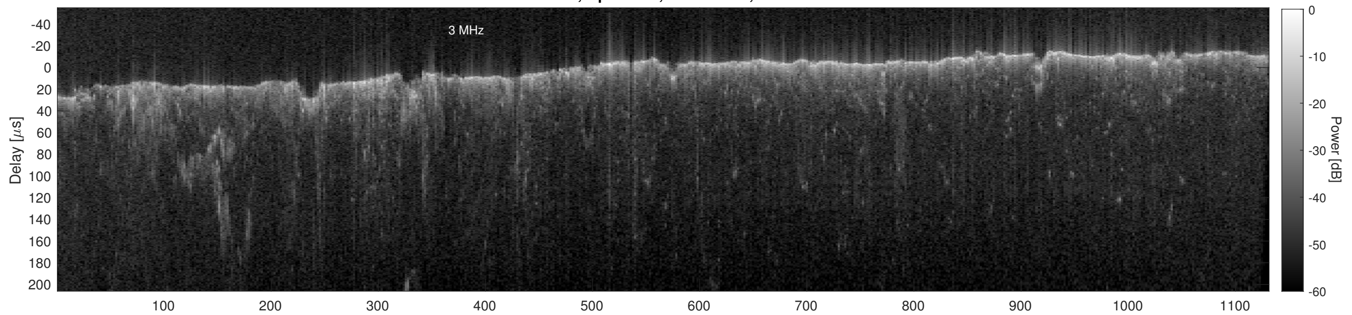
Orbit 21784, Cluttergram
