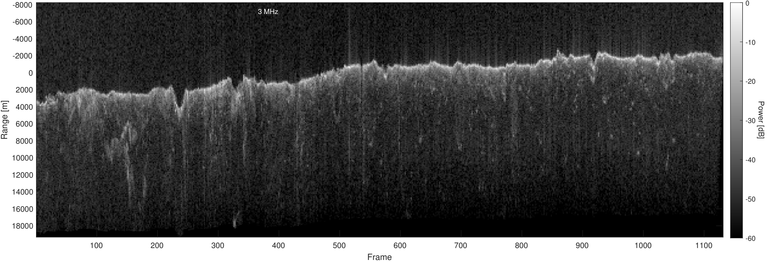
Orbit 21784, Optimized, Window, Depth-Corrected, Channel 2
