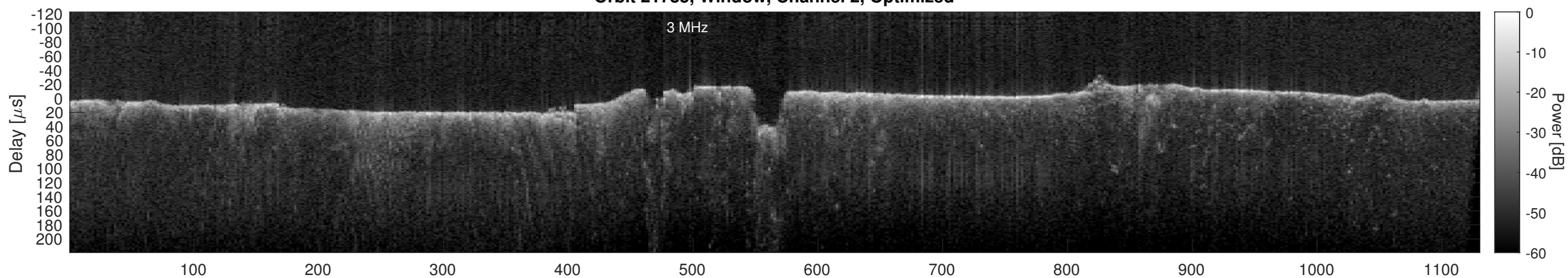
Orbit 21785, Cluttergram
