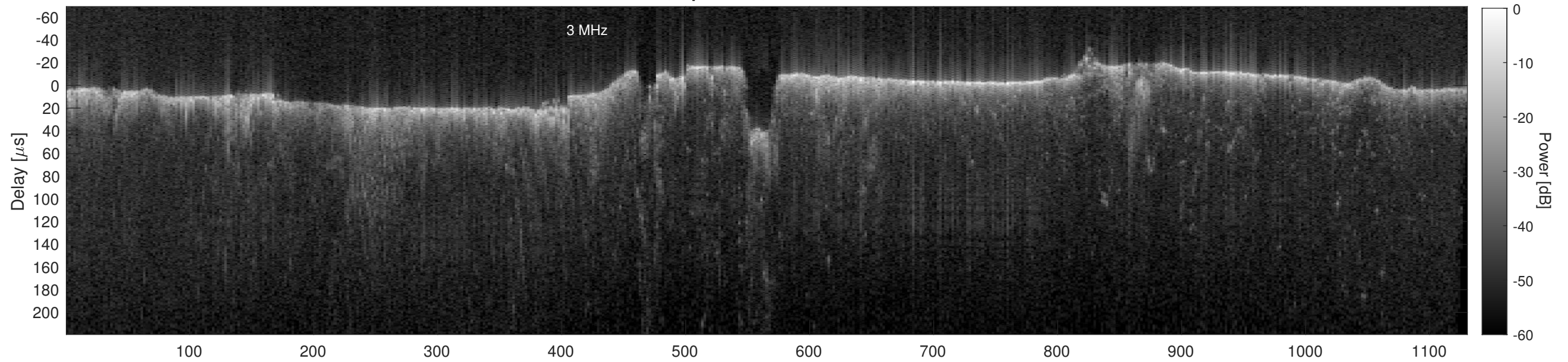
Orbit 21785, Cluttergram
