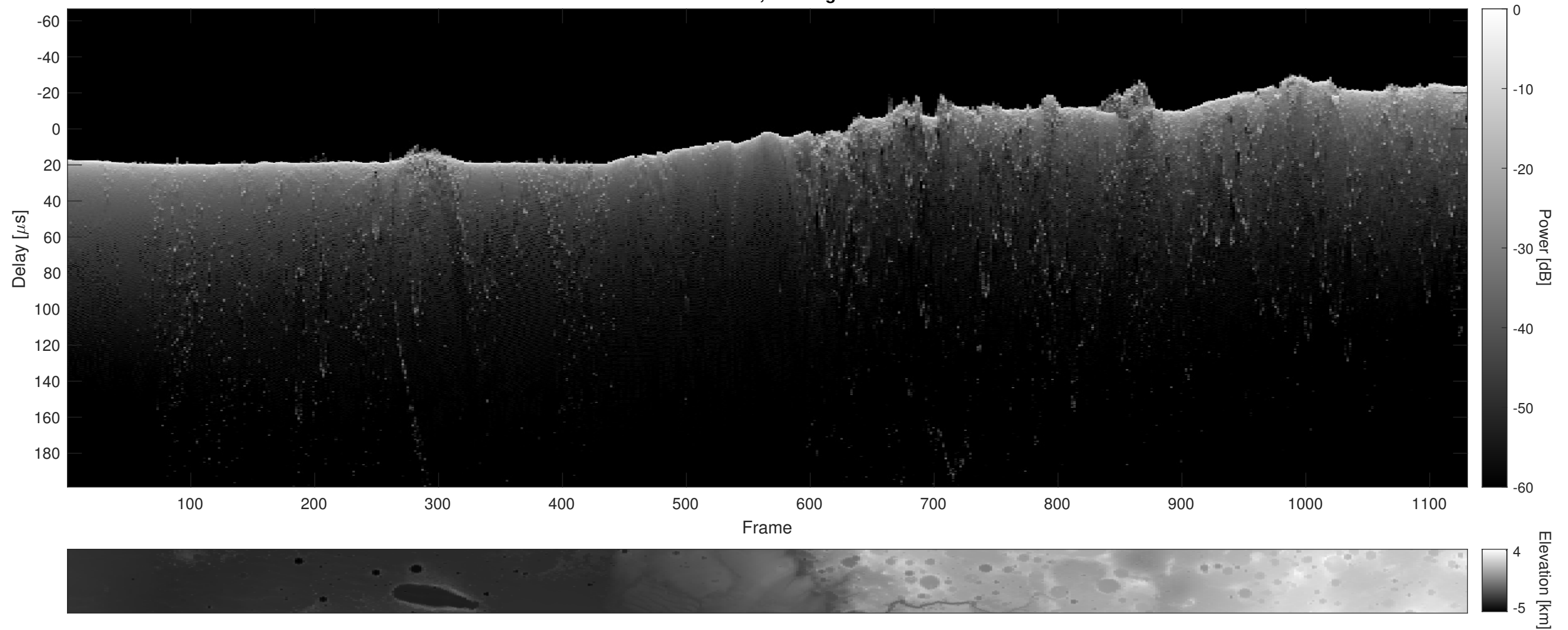
Orbit 21786, Cluttergram
