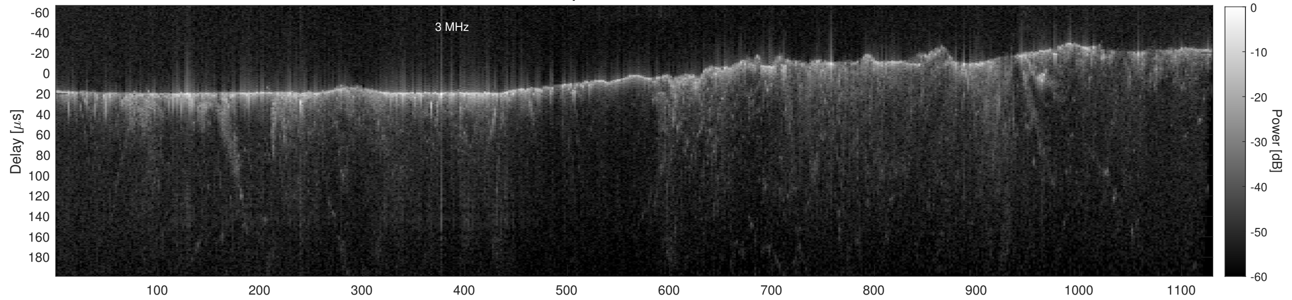
Orbit 21786, Cluttergram
