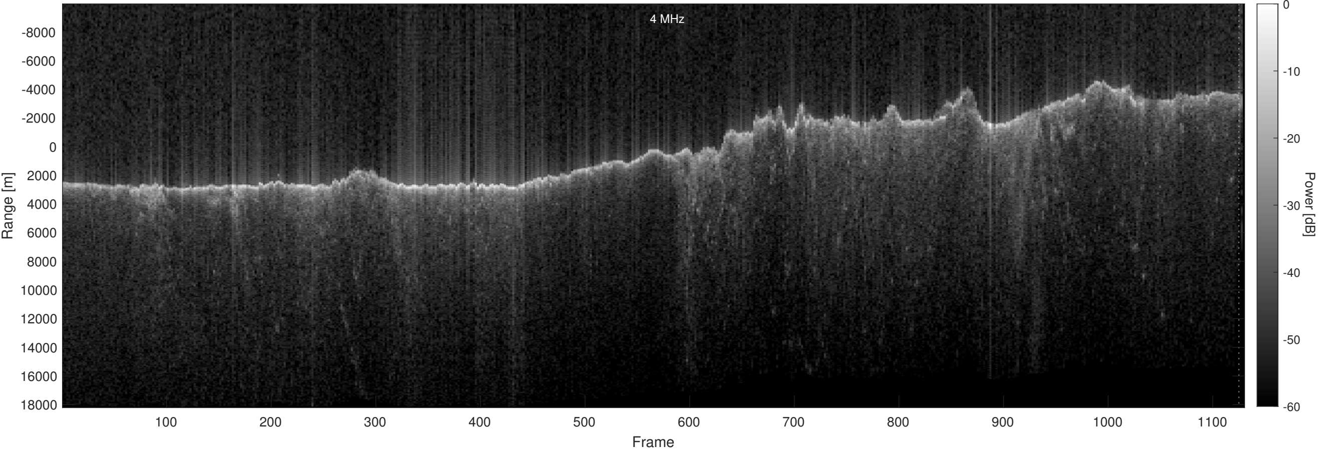
Orbit 21786, Optimized, No Window, Depth-Corrected, Channel 2
