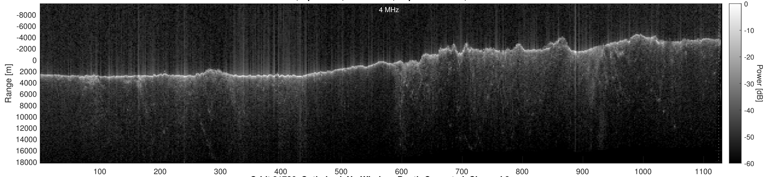
Orbit 21786, Optimized, No Window, Depth-Corrected, Channel 2
