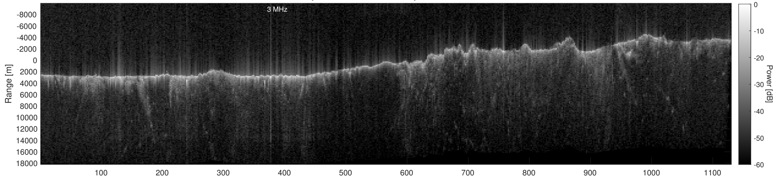
Orbit 21786, Depth-Corrected Cluttergram
