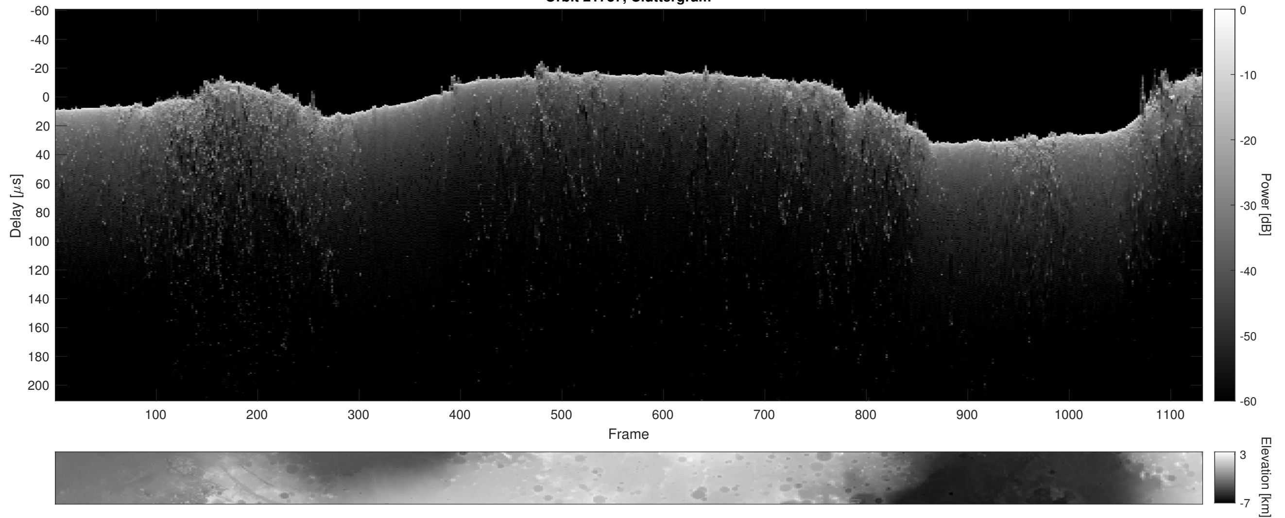
Orbit 21787, Cluttergram
