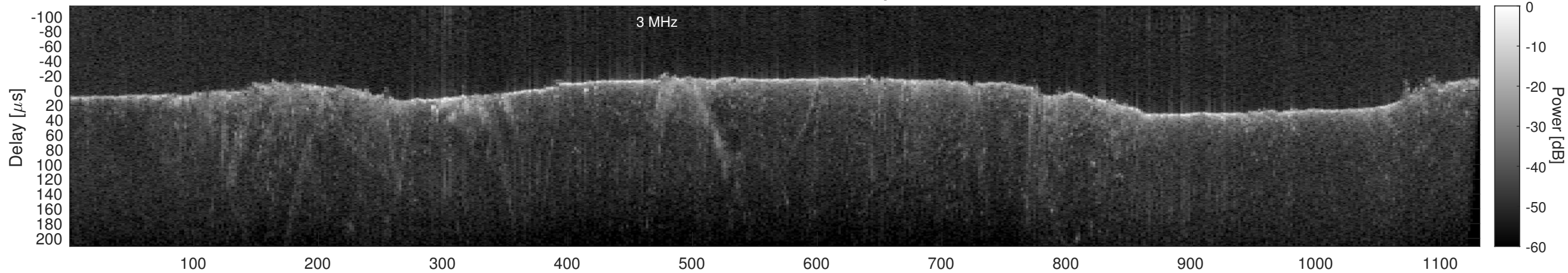
Orbit 21787, Cluttergram
