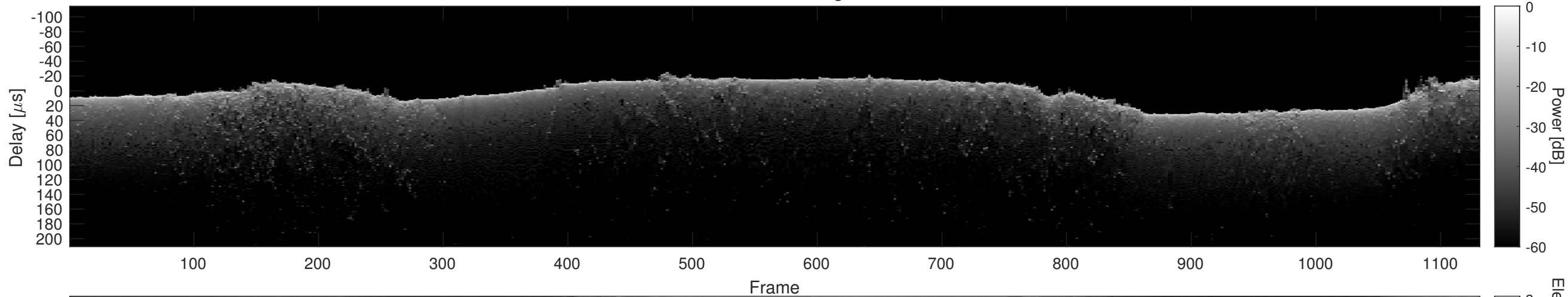
Orbit 21787, Cluttergram
