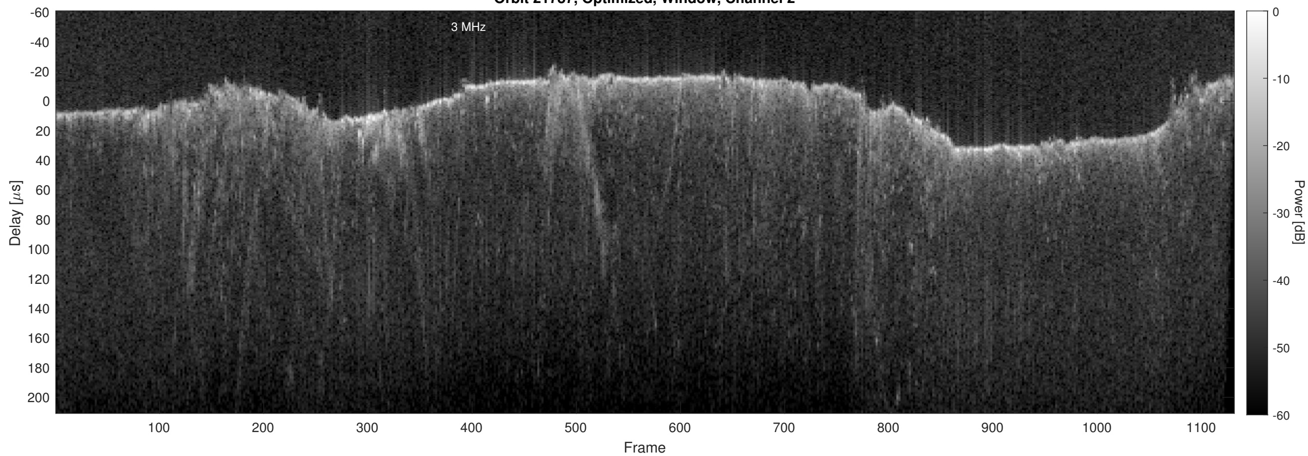
Orbit 21787, Optimized, Window, Channel 2
