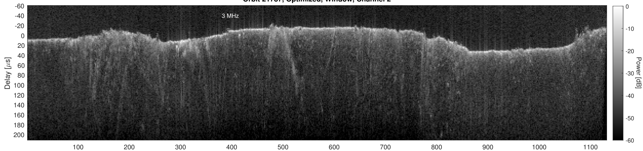
Orbit 21787, Cluttergram
