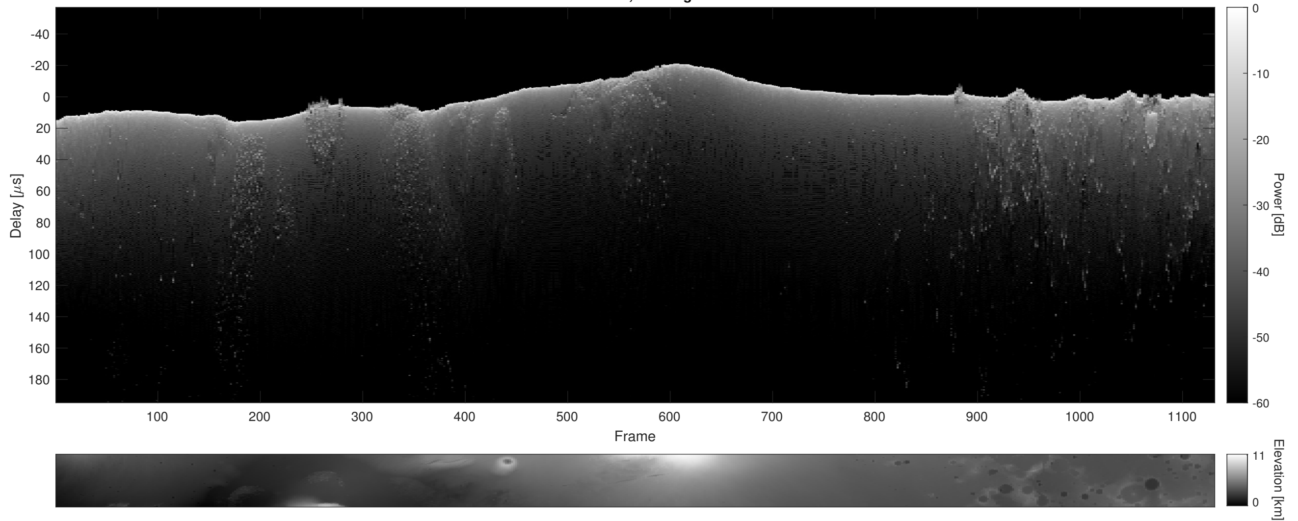
Orbit 21789, Cluttergram
