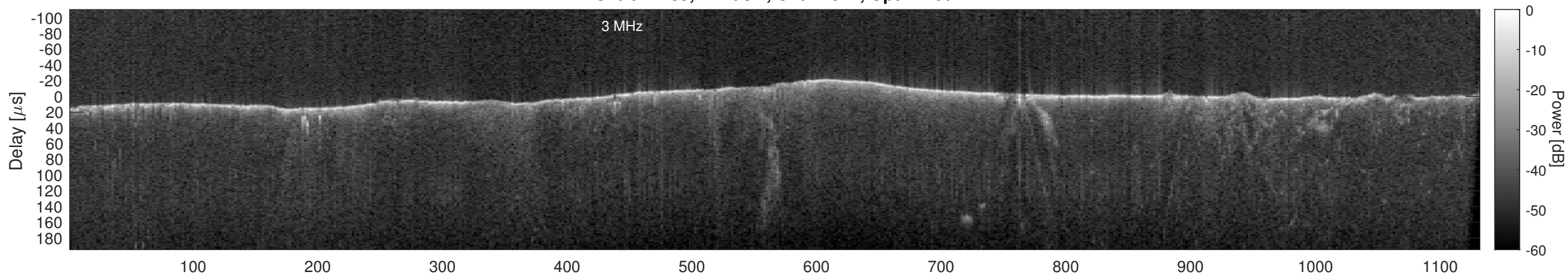
Orbit 21789, Cluttergram
