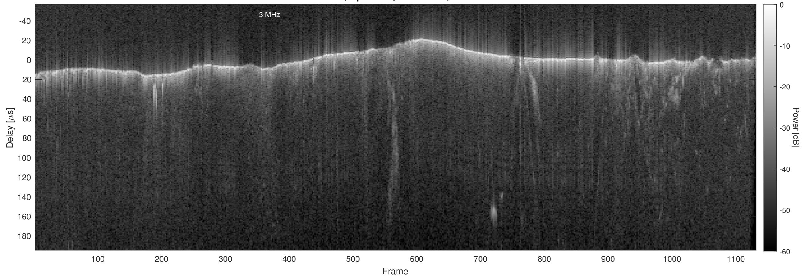
Orbit 21789, Optimized, No Window, Channel 2
